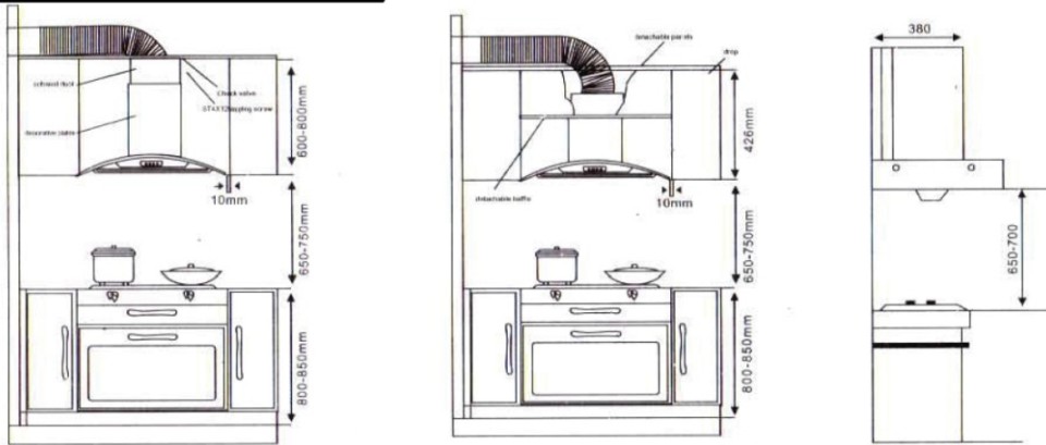
demolition back plate with the installation methods
